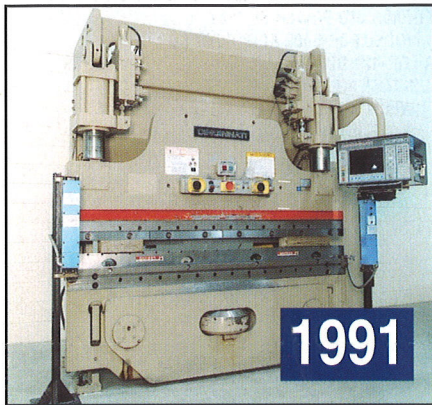
CINCINNATI MODEL 135AF 135-TON HYDRAULIC PRESS BRAKE
